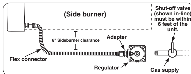
Fig. 19-3 Household propane & natural gas diagram
