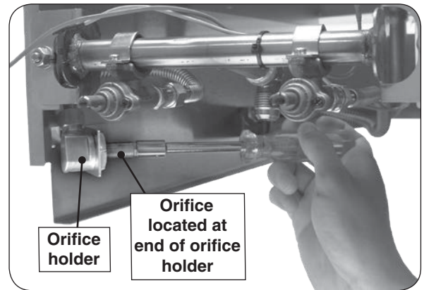
Fig. 30-1 Orifice location
