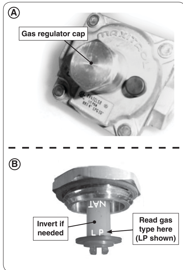
Fig. 29-1 Convert regulator
