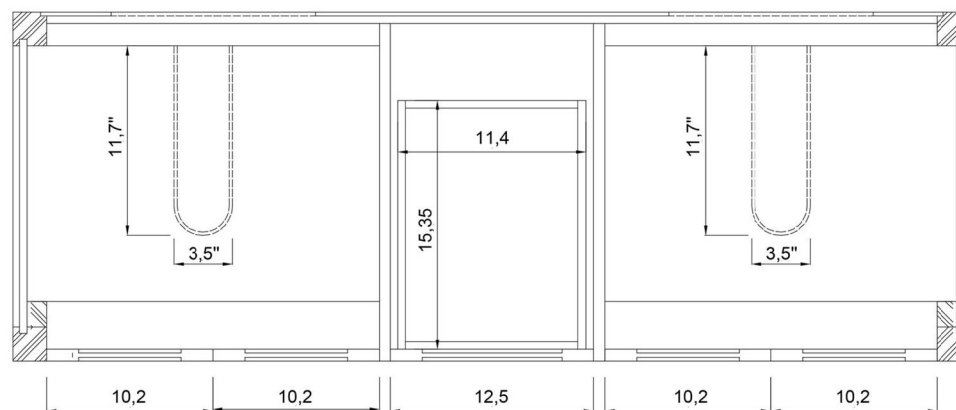
C - C SECTION
