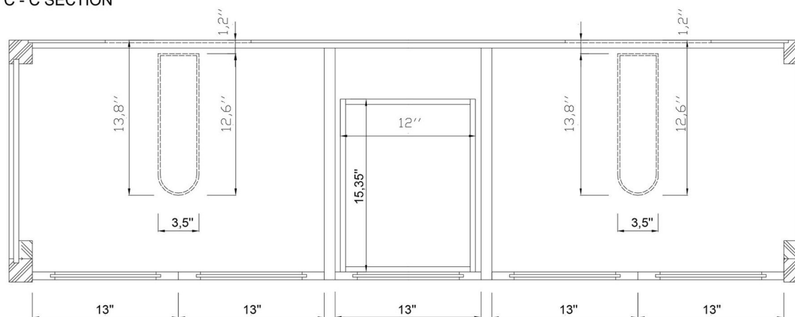
C - C SECTION
